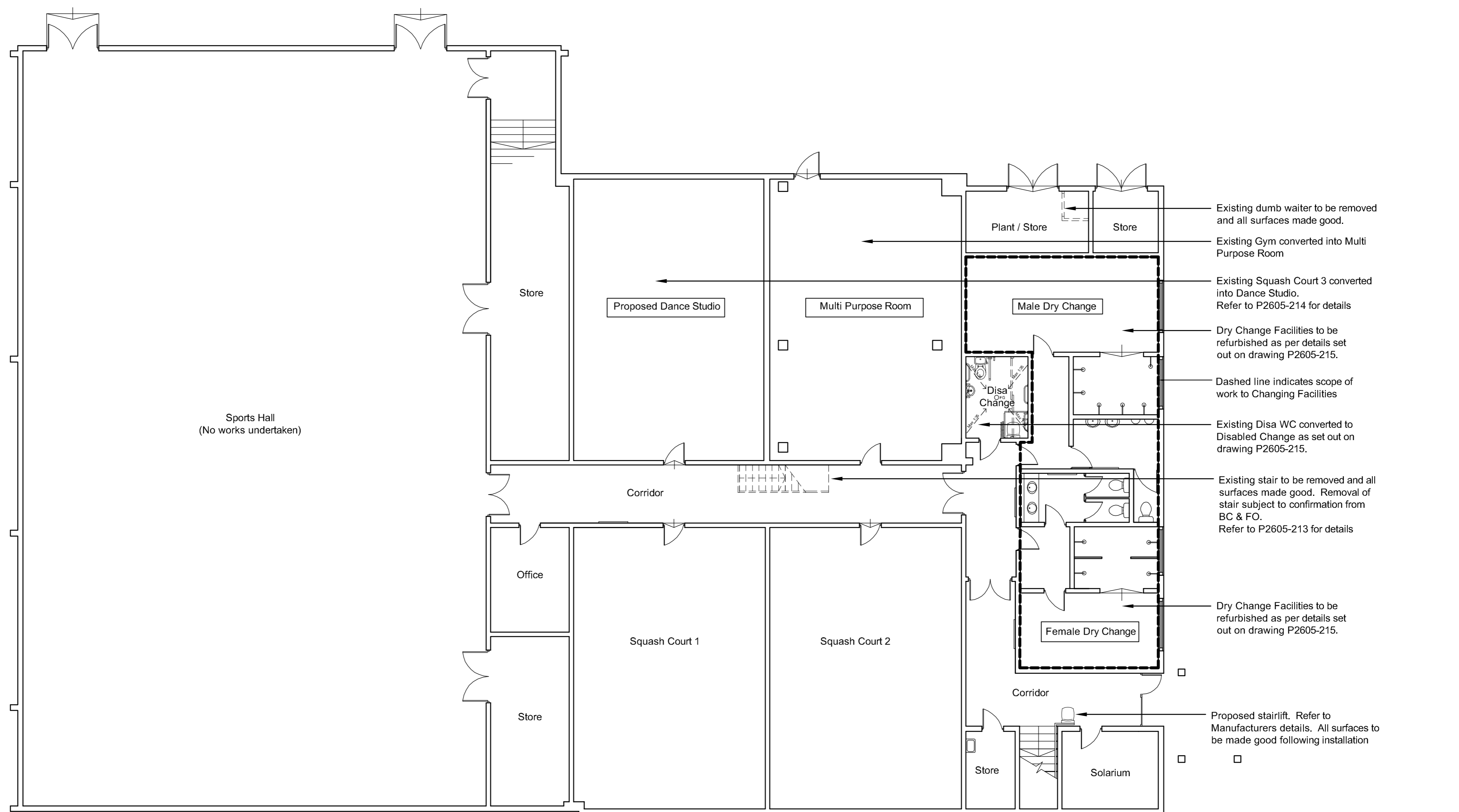
Proposed Lower Ground Floor Plan 1:100
