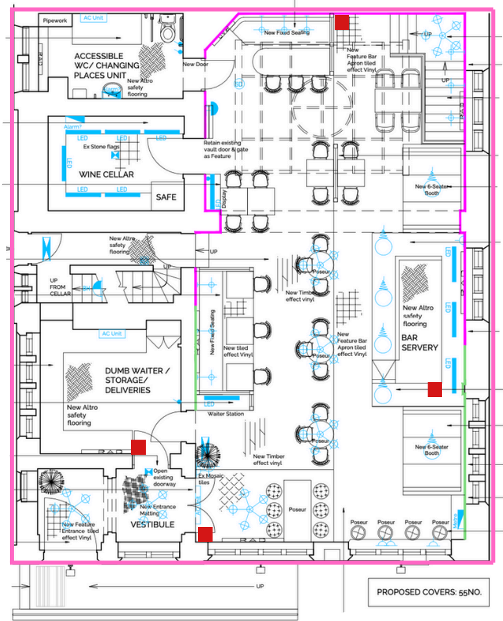
PROPOSED GROUND FLOOR PLAN - OPTION 1 SCALE 1:50
