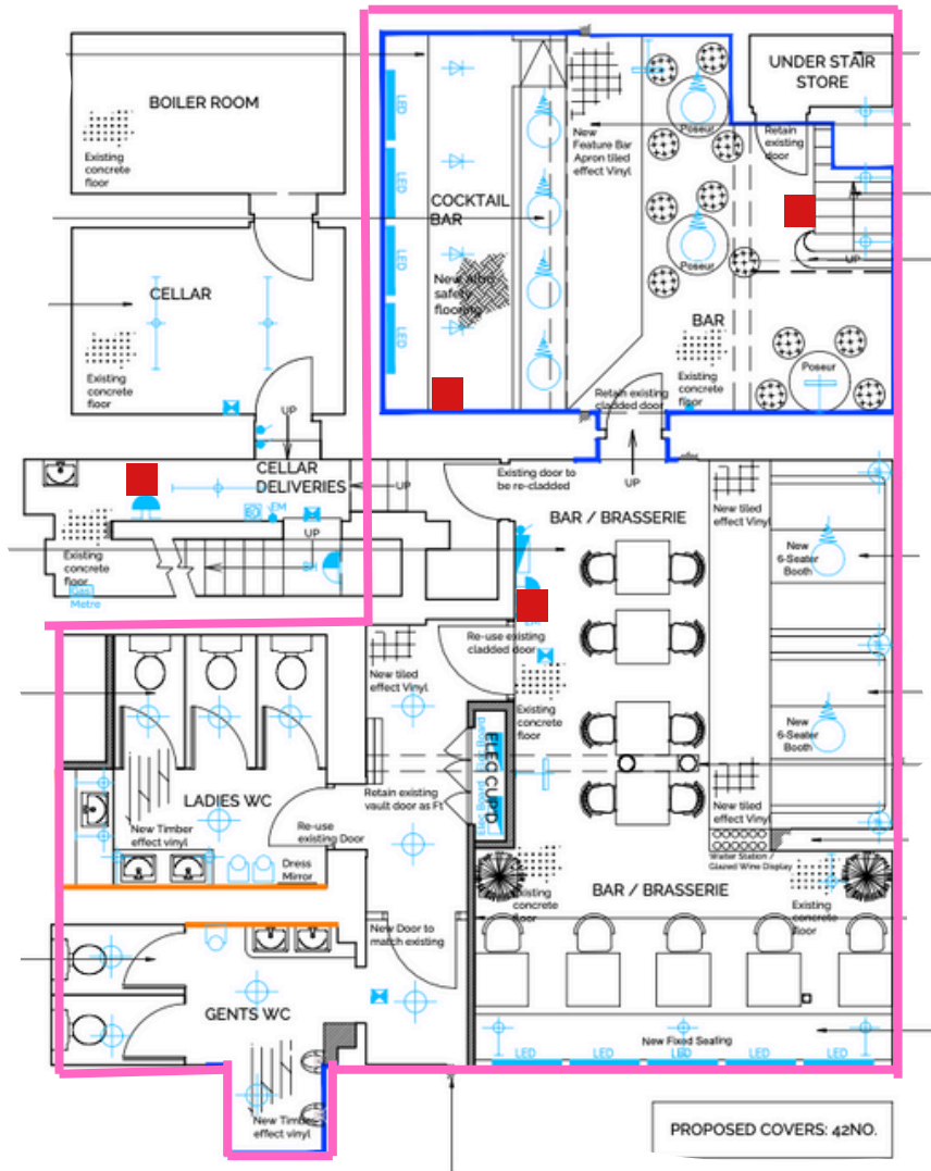
PROPOSED BASEMENT PLAN - SCALE 1:50
