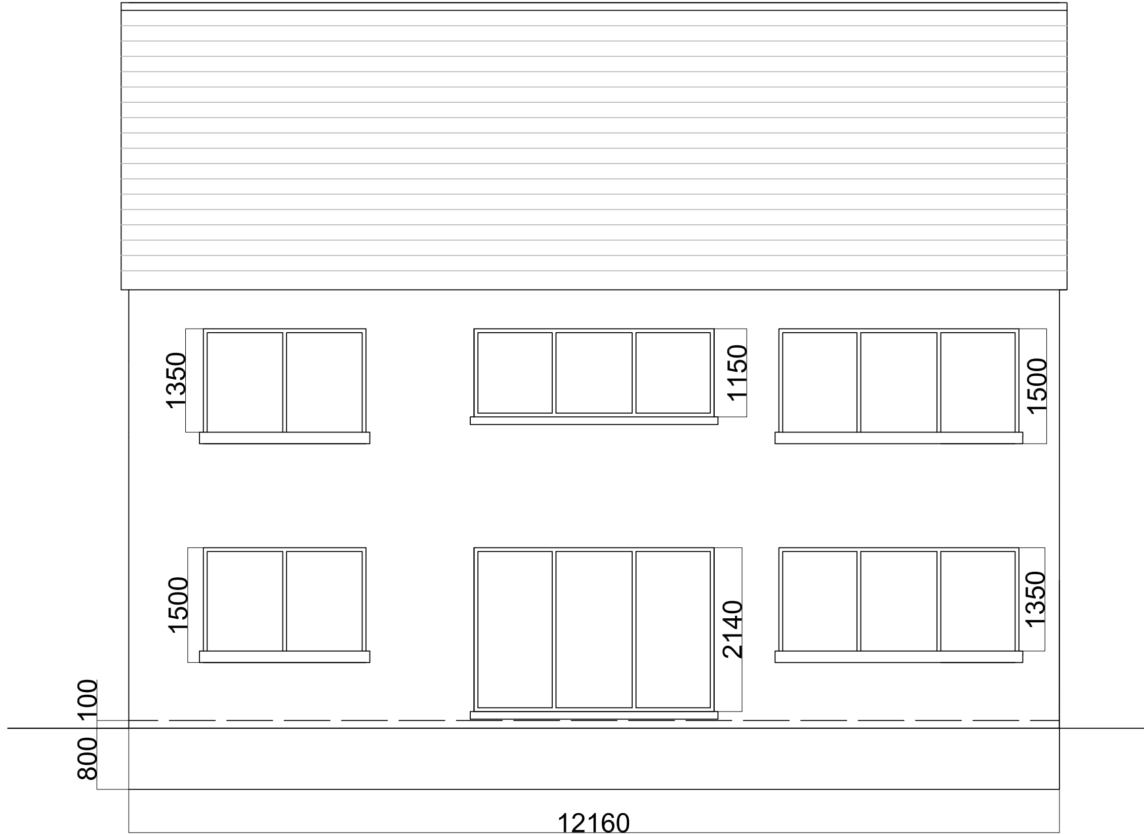
Front Elevation
