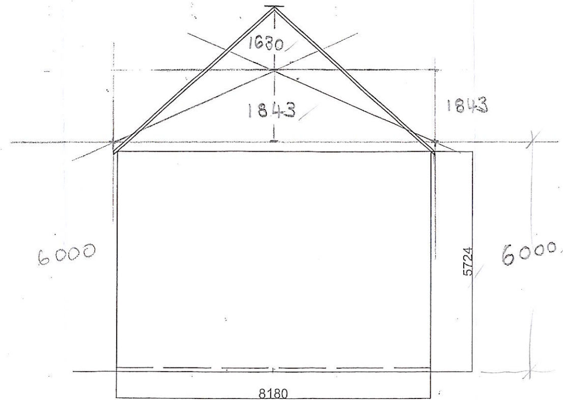
South Elevation
