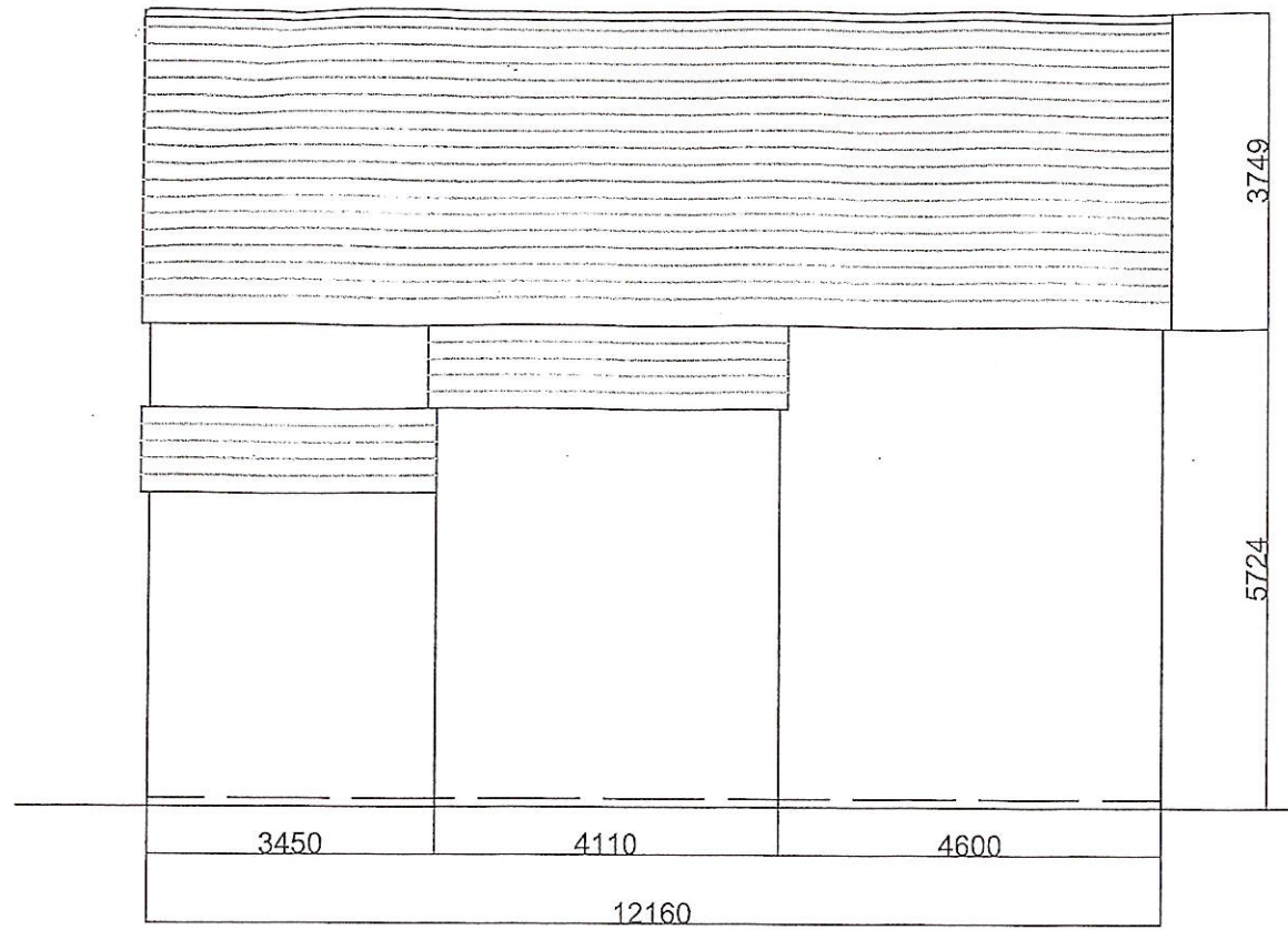
Rear Elevation
